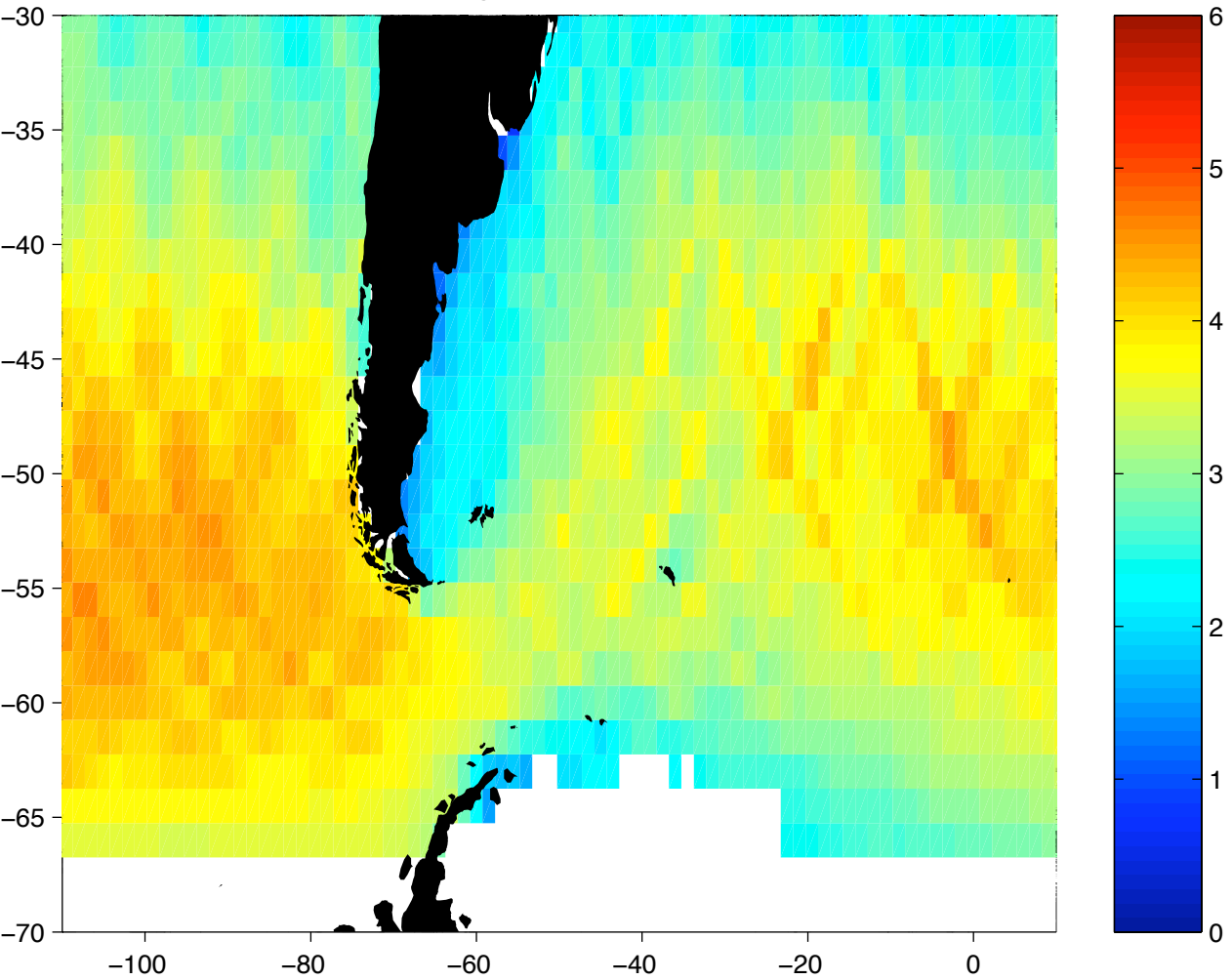
Mean Wave Height (m), April: 1993 – 2004
