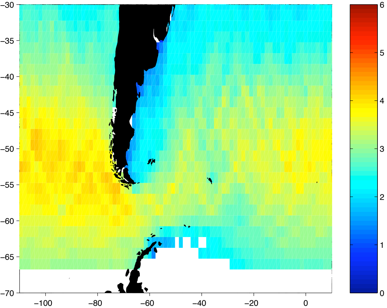
Mean Wave Height (m), March: 1993 – 2004
