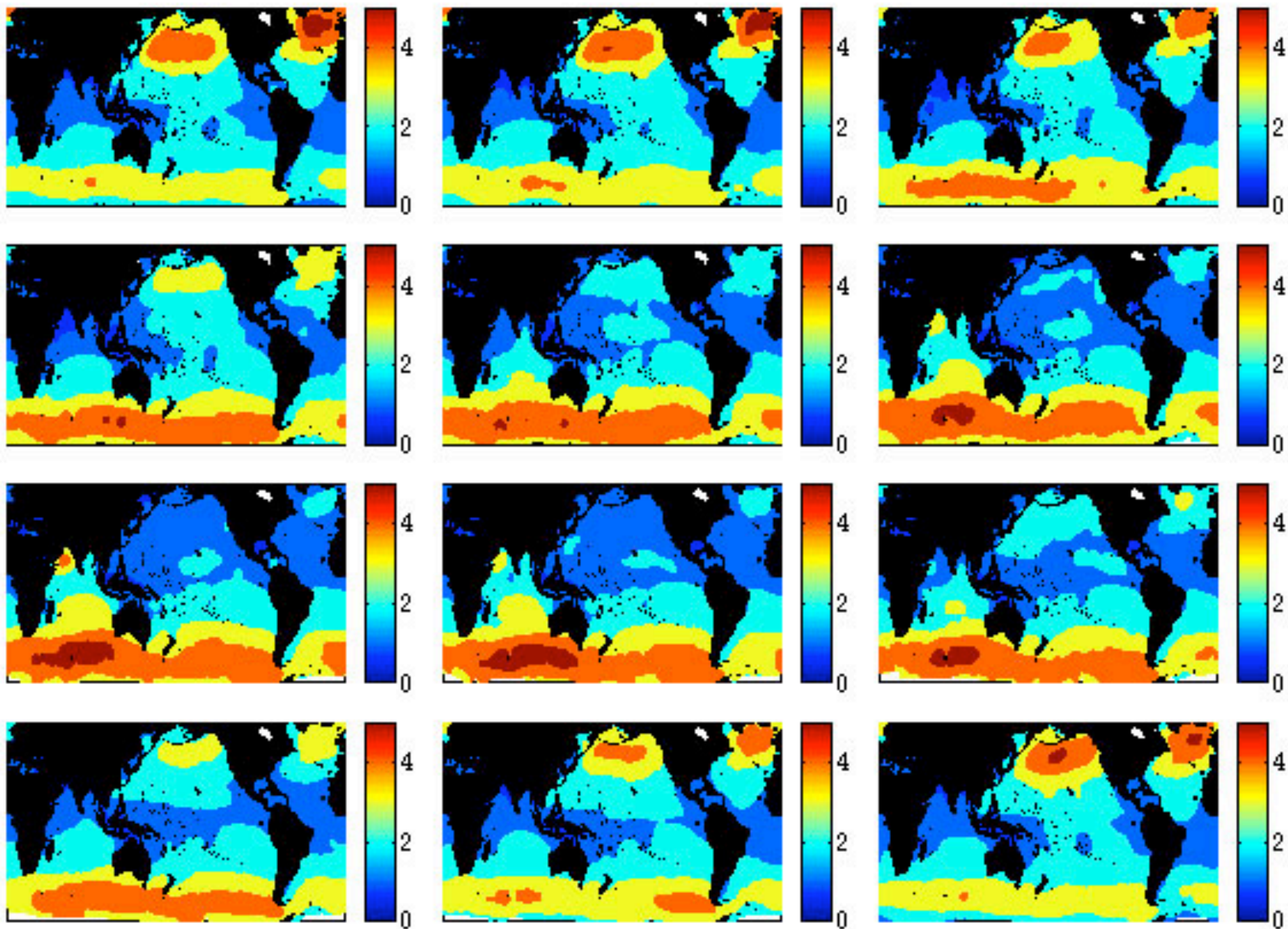
Global mean significant wave height (in meters) in the 1990s for each calendar month (January is top left).
